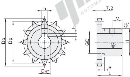
链轮 VLF02/11
