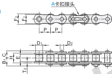
链条 VMF01/03/21
