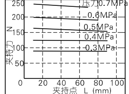
HFSZ40\HFSK40
