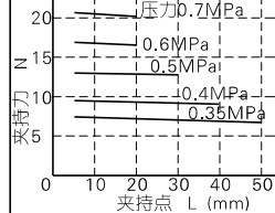
HFSZ16\HFSK16
