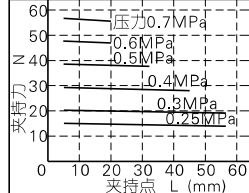
HFSZ20\HFSK20
