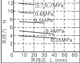
HFTZ16\HFTK16
