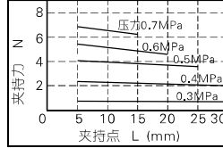
HFSZ10\HFSK10
