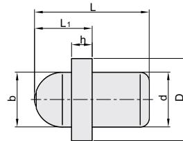
油嘴形状
