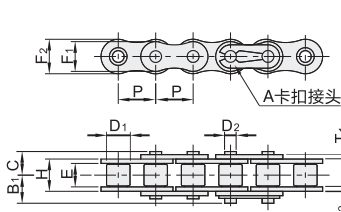
链条 VMC01/11
