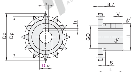
链轮 VLY21/22
