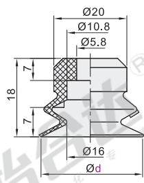
盘径Ø70
