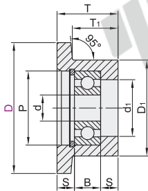
单列轴承 QBR81/82
