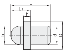
油嘴形状
