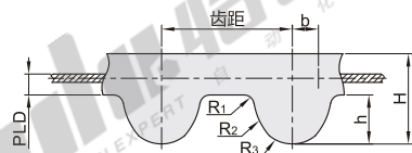
◎ ECE35-3GT (齿距: 3)
