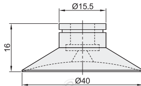
盘径Ø40
