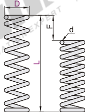
□ YUM/E-YUM/J-YUM 允许位移量 F_{max}=L \times (28-35)\%
