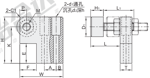
旗型限位块+聚氨酯螺钉 ICR45
