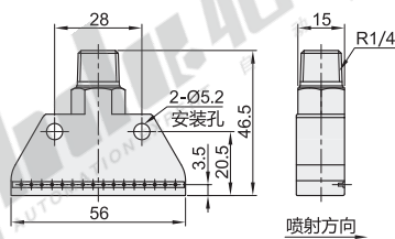
紧凑型·垂直式喷射(ABS) NHR89
