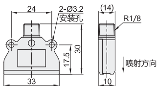
超小型·平行式喷射(ABS) NHR85
