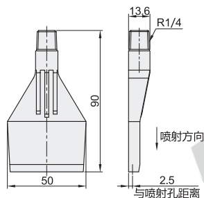
紧凑型·平行式喷射(ABS) NHR75
