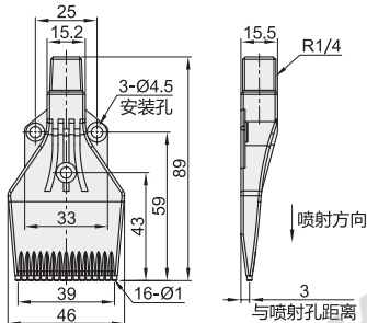
标准型·平行式喷射(ABS) NHR71
