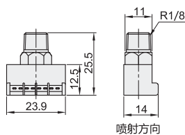
紧凑型·垂直式喷射(ABS) NHR89
