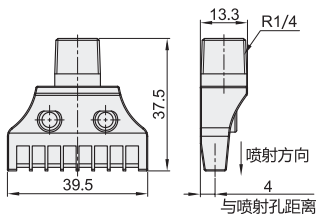
紧凑型·平行式喷射(ABS) NHR75
