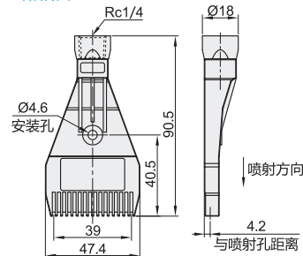
标准型·平行式喷射(ABS) NHR74
