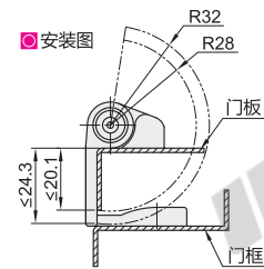
HFS23(锥孔+定位柱型)
