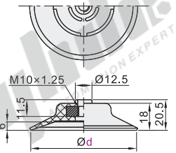
盘径Ø80
