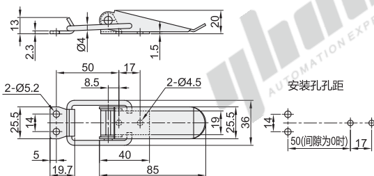
HFQ52
