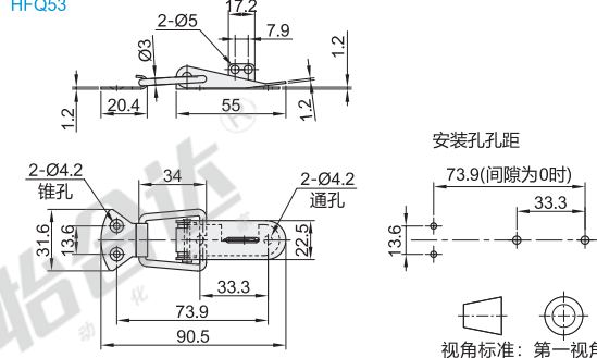
HFQ53
