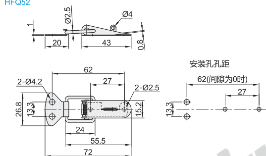
HFQ52
