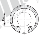
挡圈装配尺寸
