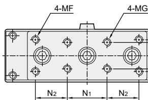
(滑塊視圖)
