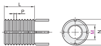
4根插销适用M8-M16
