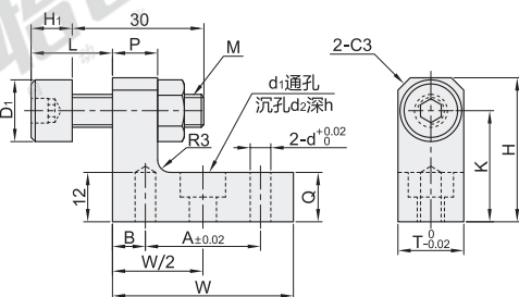
紧凑型限位块+聚氨酯螺钉
