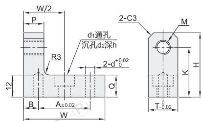
紧凑型限位块+聚氨酯螺钉
