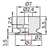
盘径Ø8
