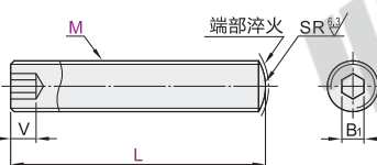
内六角孔型 PAS11/12/13/14/15/16/17/18/19/20/21/25/26/30
