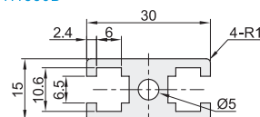
AOB02-H1530B AOB05-H1530B AGB06-H1530B
