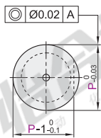
圆型 YKD21/22/23
