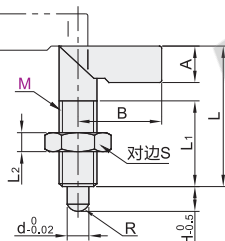
带锁紧螺帽 ZAU21/22
