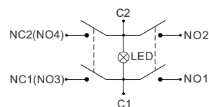
6脚 (3档) 原理图 Schematic diagram of 6-pin (3rd gear)
