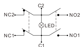
6脚 (2档) 原理图 Schematic diagram of 6-pin (2nd gear)
