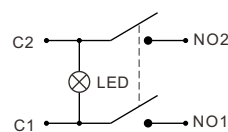
4脚 (2档) 原理图 Schematic diagram of 4-pin (2nd gear)
