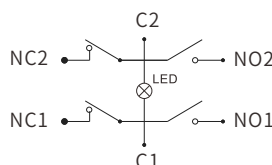
带灯 (2档/6脚) With LED (2 Gears/6PINS)
