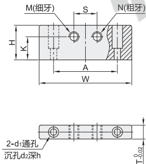
方型限位块 ICR80/81/82
