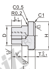
WHL51/52
