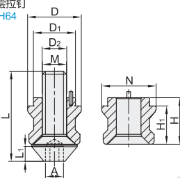
补偿拉钉 ZFH64
