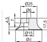
盘径Ø40
