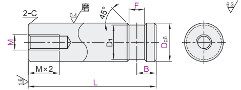
一端带止动螺丝槽一端内螺纹型 SHT21/22/26/27
