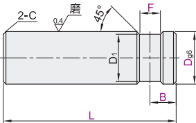
一端带止动螺丝槽 SHT01/02/06/07
