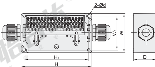
极数: 15P/20P
