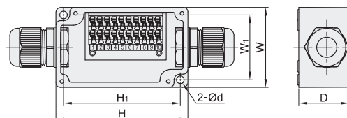
极数: 15P/20P
