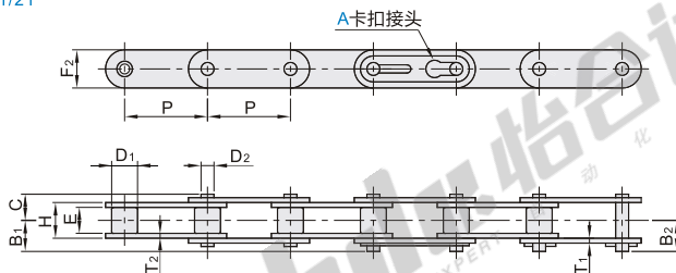
双节距小滚子输送链条 VMM01/11/21
