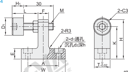
凸型限位块+聚氨酯螺钉 ICP54
