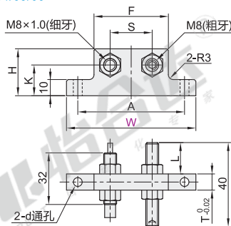
宽幅凸型限位块+缓冲调节 ICP64/65/66
