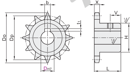
双节距小滚子输送链轮 VLM01/11/21
