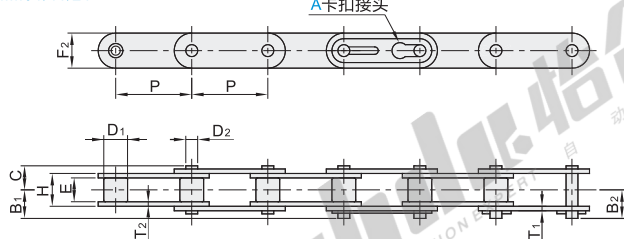
双节距小滚子输送链条 VMM01/11/21
