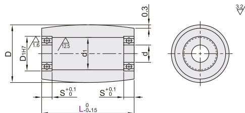
圆弧形 QAC11/12/31/51
