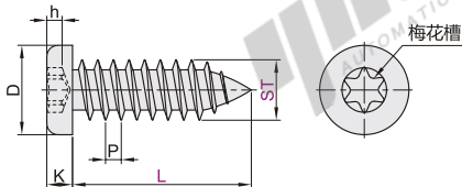
梅花槽盘头自攻螺钉 TBS60
