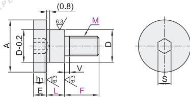
短头型 MJT21/22/26/31/32/36
