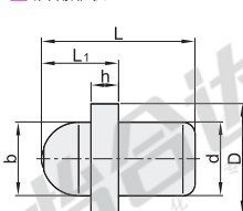
油嘴形状
