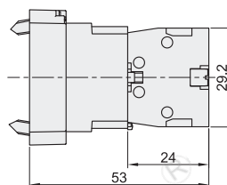
带灯 ZHC63
