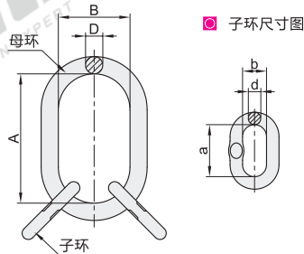
G100起重子母环 TCE02
