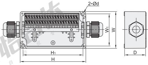
极数: 15P/20P
