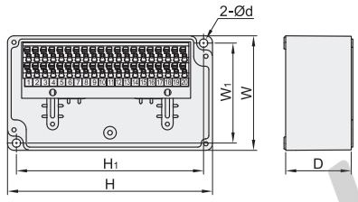
极数: 15P/20P
