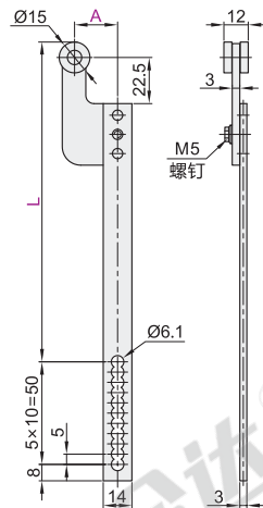
带圆眼多孔连杆 XAV56
