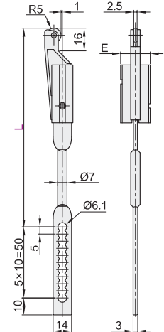
带滚轮连杆 XAV61/62
