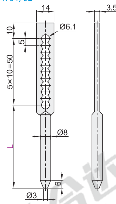
带多孔连杆 XAV51/52
