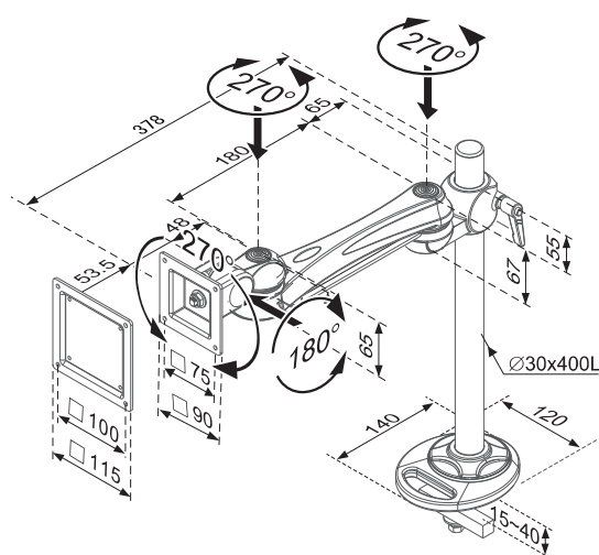
LA-52-6 Clamp Type
