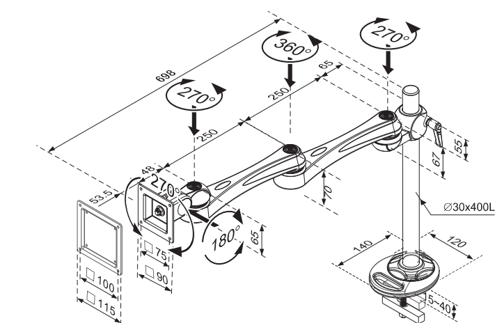
LA-52-5 Clamp Type
