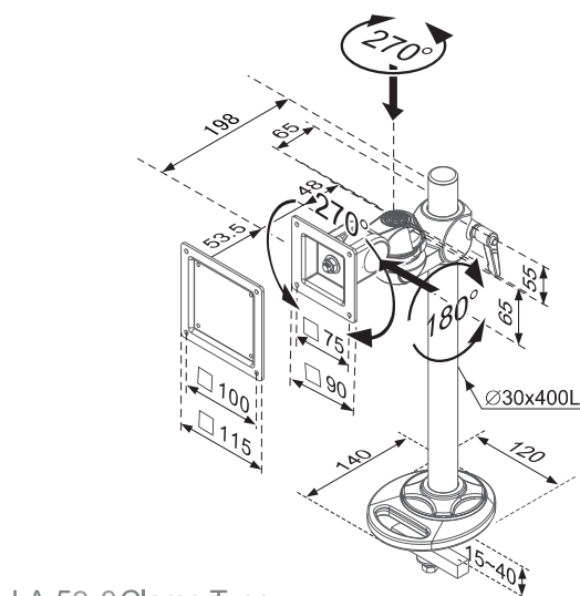
LA-52-3 Clamp Type
