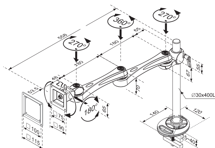
LA-52-4 Clamp Type
