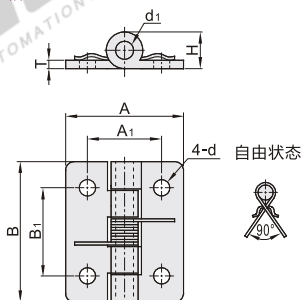
HFG41/51 规格: 40/50
