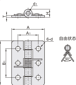
HFG41/51 规格: 65/75
