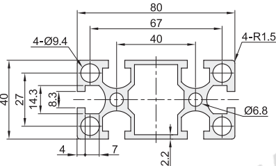
AGB06-J4080Y
