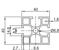
AGB06-J4040GA
