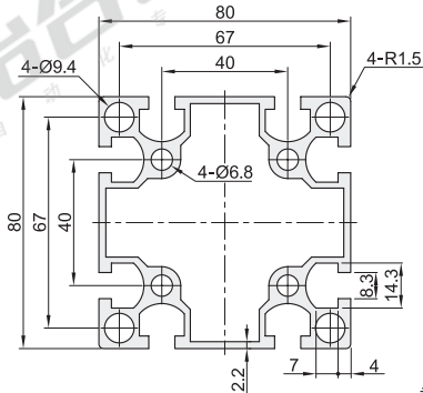
AGB06-J8080Y
