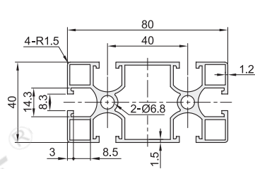
AGB06-J4080A
