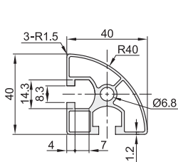
AGB06-J4040RS
