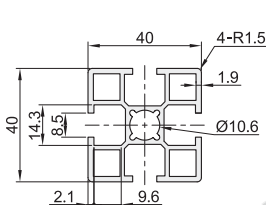
AGB06-J4040G
