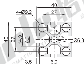
AGB06-J4040GY
