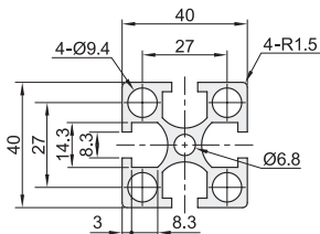
AGB06-J4040G
