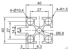
AGB06-J4040GY
