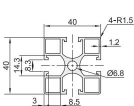
AGB06-J4040GA
