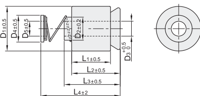
带弹簧 HCA12
