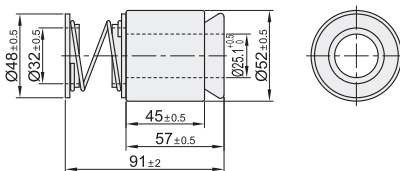
带弹簧 HCA14
