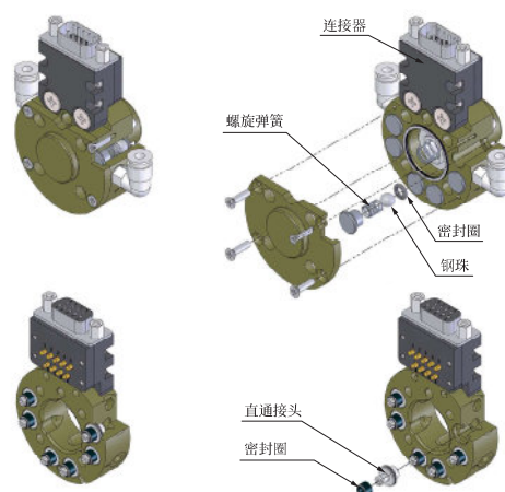
OX-03A(05A,10B)/03A(05A,10B)I
