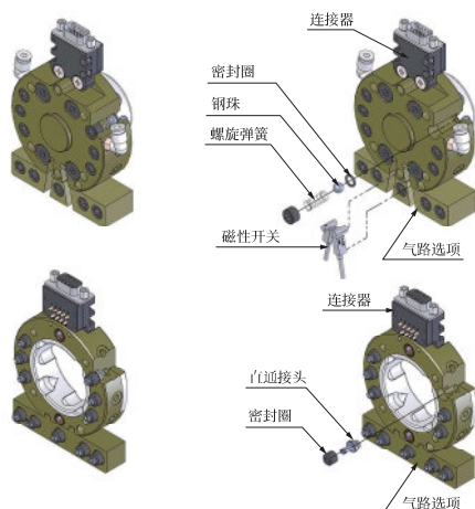
OX-20B/20BI
