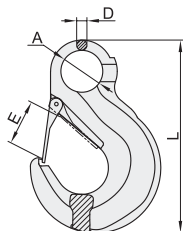
G80眼型滑钩 TCD31
