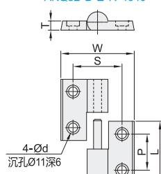
AKQ52-B-Z-R-4040
