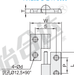
AKQ52-B-Z-R-3030
